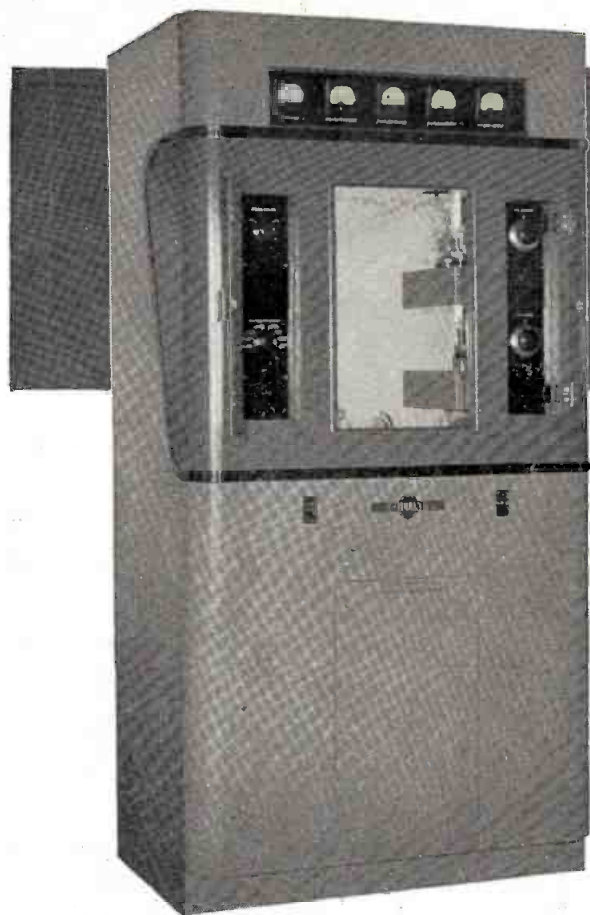
Front view of 20V with doors at both sides open for access to power change, PA loading, PA tuning and multimeter controls.
